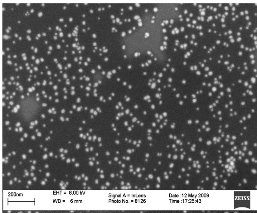
Fig. 2. Scanning electron micrographs of the prepared AuNPs. One drop of AuNPs was placed on silicon slide and left to dry then examined using field emission scanning electron microscopy (Model: Leo Supra 55).
