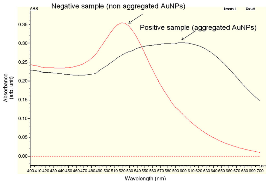
Fig. 4. Extinction spectra of positive and negative samples. The absorption spectra of positive sample (aggregated AuNPs, black) and negative sample (non-aggregated AuNPs, red). Note the red shift and broadening of the peak of the positive sample due to aggregation of AuNPs. For the negative sample, the \lambda_{\max} was around 518–520 nm.
