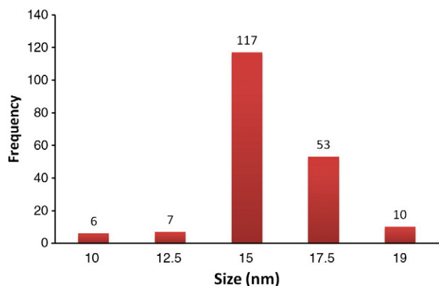
Fig. 3. Analysis of AuNPs size distribution. The scanning electron microscope image in Fig. 2 was analyzed by Image J 1.4 software Wayne Rasband, National Institutes of Health, USA. http://rsb.info.nih.gov/ij/java 1.6.0_05 .
